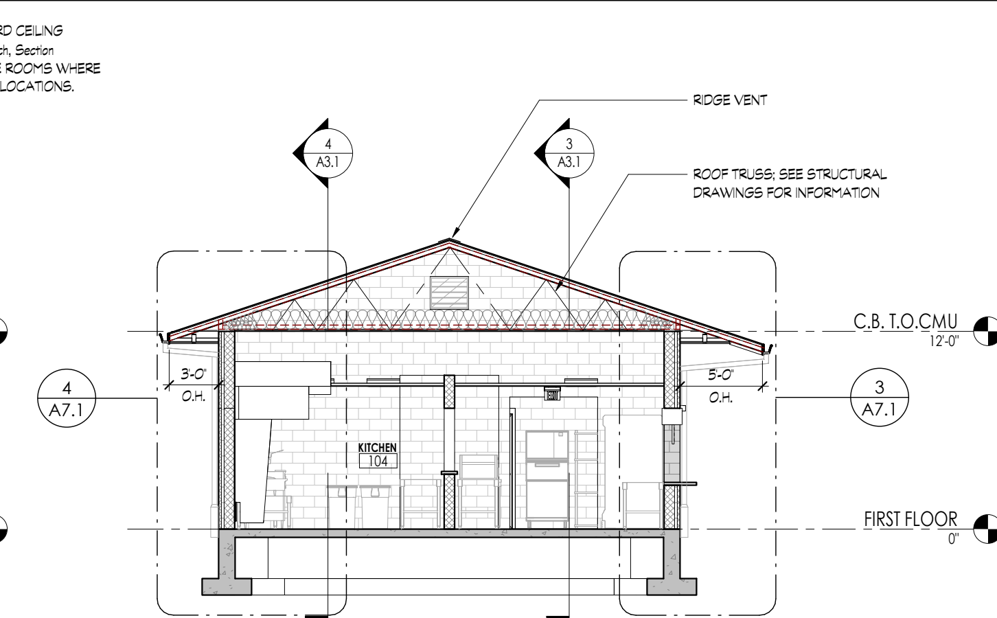
7) FIELD HOUSE BUILDING - TRANSVERSE SECTION C 1/8" = 1'-0"
