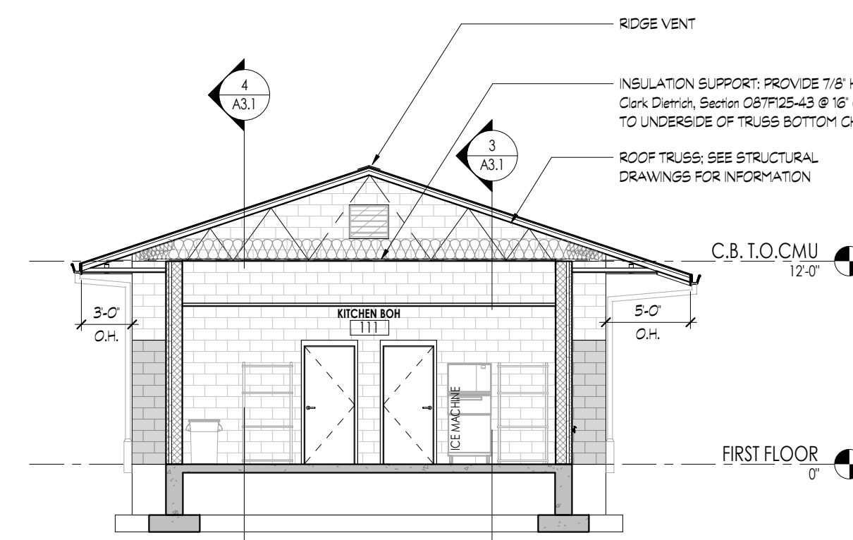
8) FIELD HOUSE BUILDING - TRANSVERSE SECTION D 1/8" = 1'-0"
