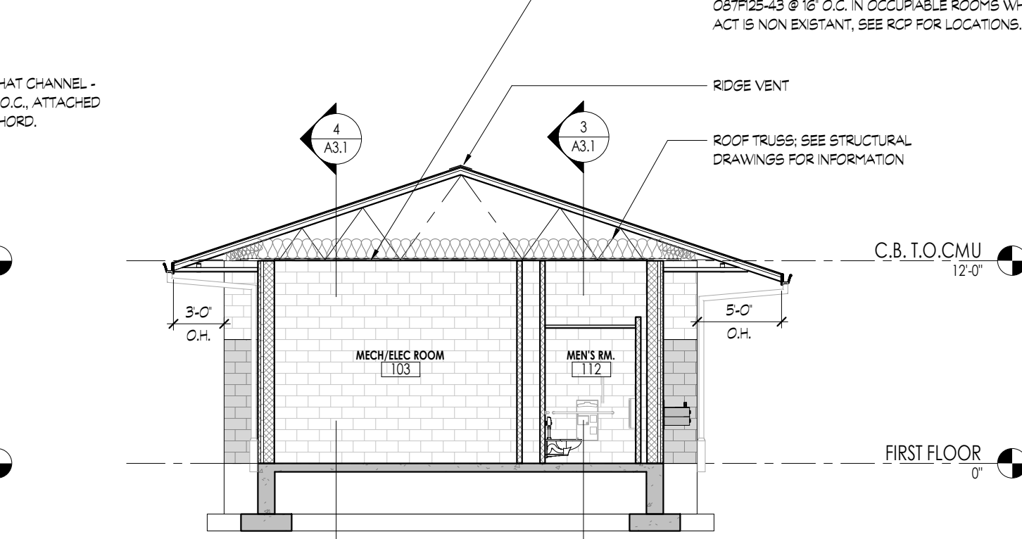
6) FIELD HOUSE BUILDING - TRANSVERSE SECTION B 1/8" = 1'-0"
