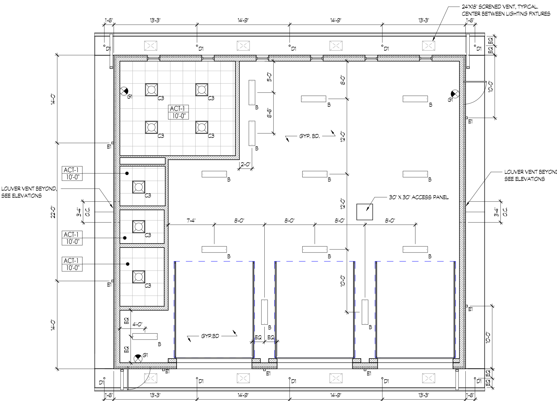
2) GARAGE BUILDING - FIRST FLOOR RCP 1/8" = 1'-0"
