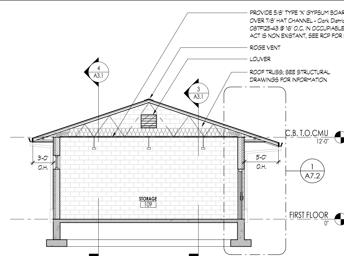
9) FIELD HOUSE BUILDING - TRANSVERSE SECTION E 1/8" = 1'-0"
