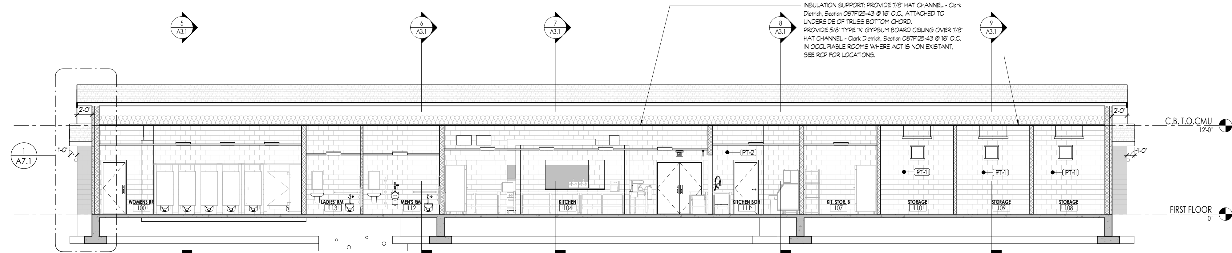
3) FIELD HOUSE BUILDING - LONGITUDINAL SECTION A 1/8" = 1'-0"
