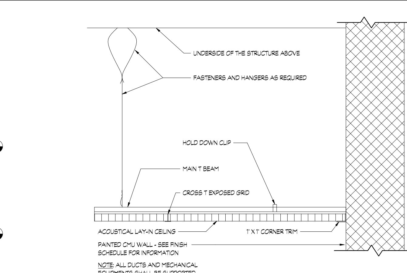
5) FIELD HOUSE BUILDING - TRANSVERSE SECTION A 1/8" = 1'-0"
