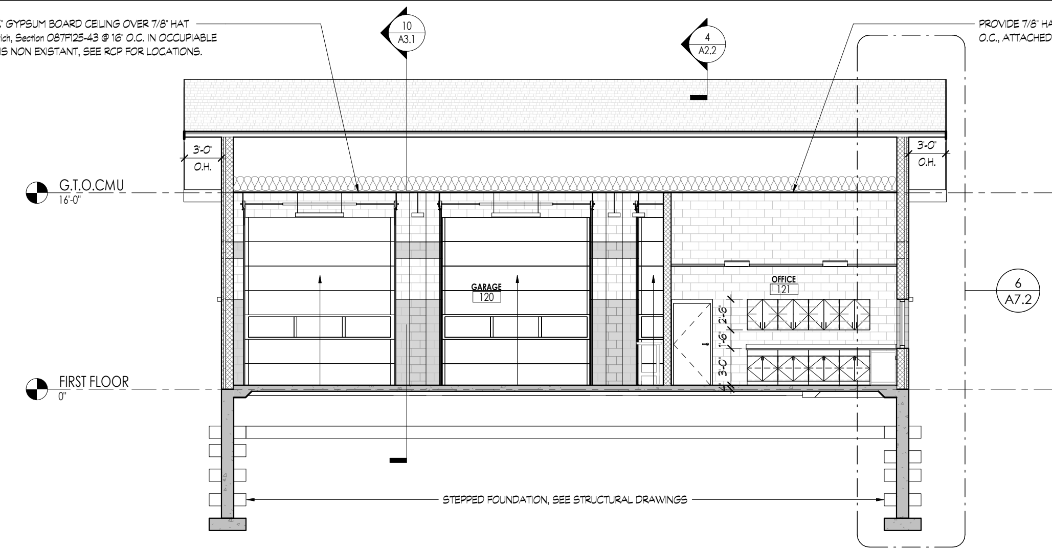
11) GARAGE BUILDING SECTION B 1/8" = 1'-0"
