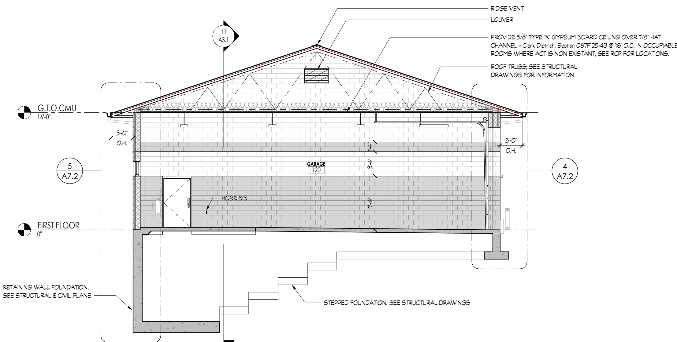
10) GARAGE BUILDING SECTION A 1/8" = 1'-0"
